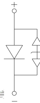
Fig.1-4 Polarity
