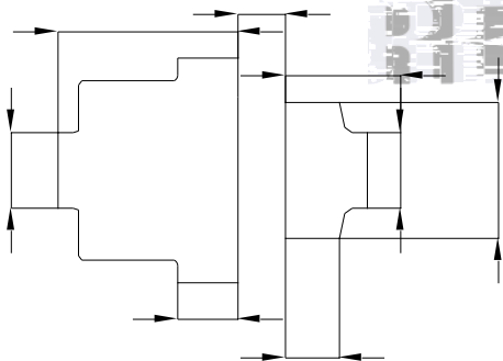
Fig.1-5 Soldering Patterns
