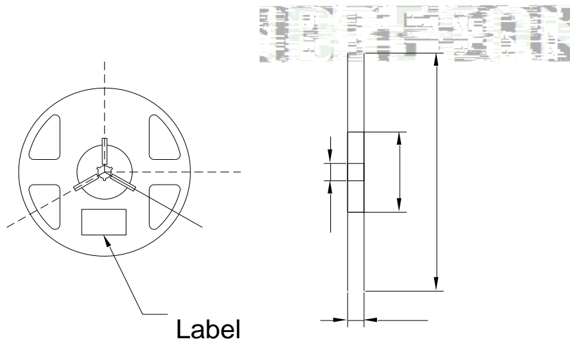
Fig.2-2 Reel Dimension
