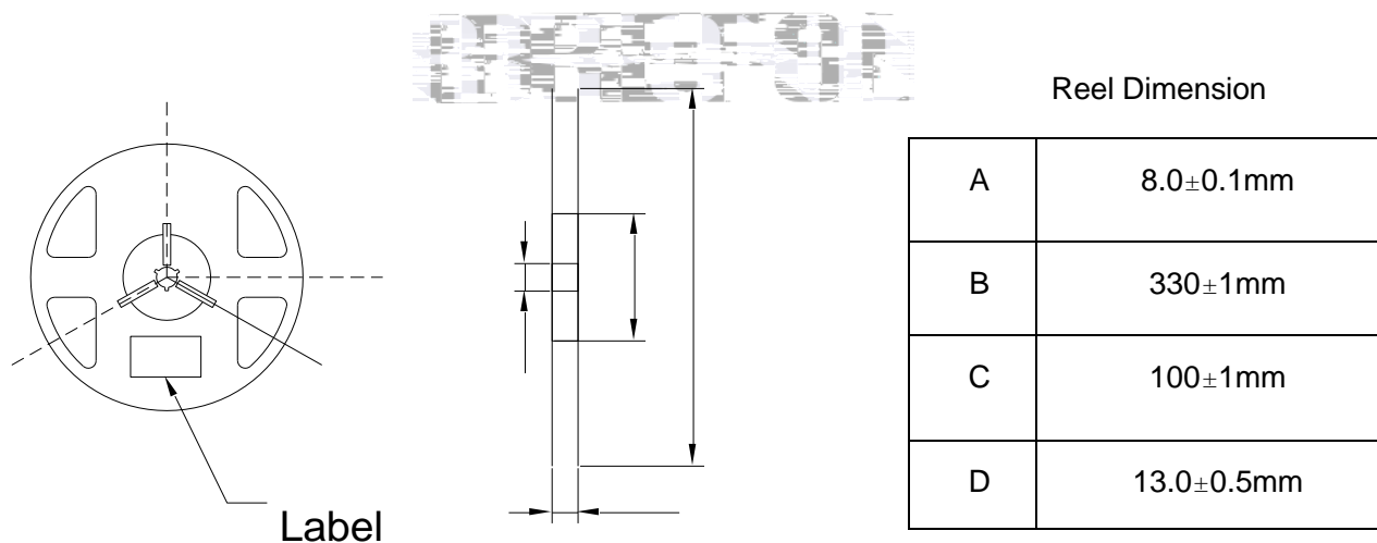
Fig.2-2 Reel Dimension
