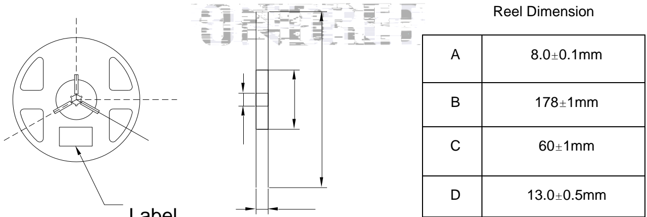
Fig.2-2 Reel Dimension
