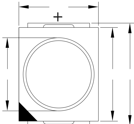
Fig.1-1 Top View
